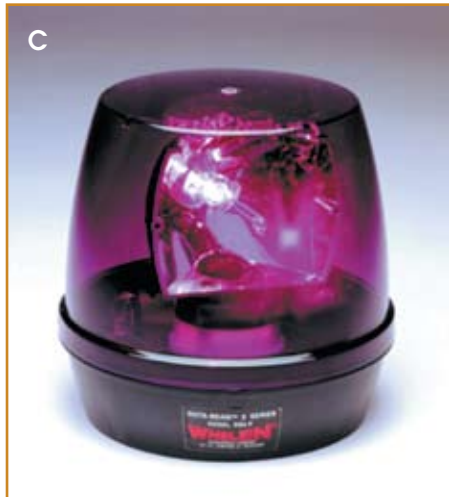
C. ROTA-BEAM 6 HALOGEN Single reflector, 50 watt halogen lamp dome. Quiet, two-ball-bearing rotator assembly. Magnetic mount includes 50# pull magnet, 8 ft. power cord with cigarette lighter plug. Input voltage/current draw: 12.8 VDC, 4 amps. 6.75"H x 6.1875" Dia., 1 lb. 3-year warranty on motor. Easily converts to permanent mount. Please specify blue, amber, purple or red. 576524
